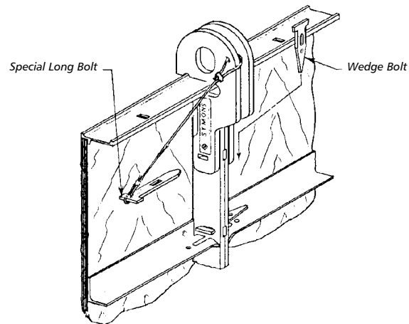
Double Duty Lift Bracket Attachment
