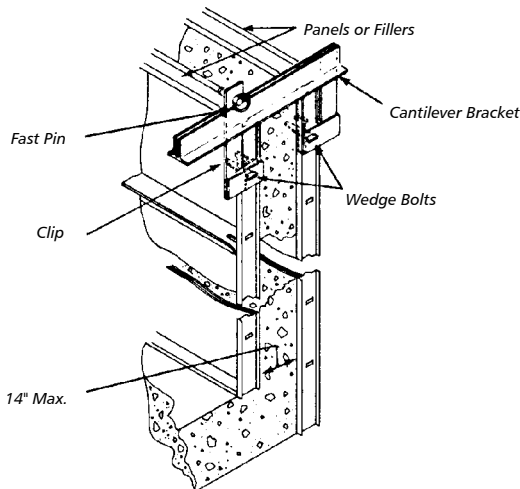
Cantilever Bracket Attachment
