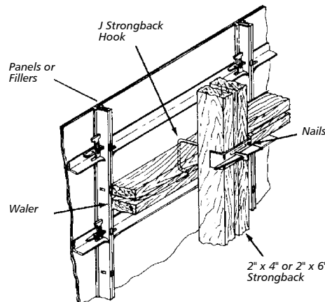
Strongback Attachment
