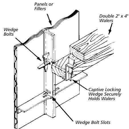
Z-Tie Holder Attachment
