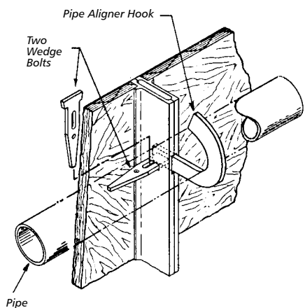
Typical Pipe Alignment
