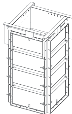
Adjustable Column Extender
