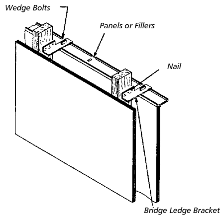
Brick Ledge Bracket Attachment
