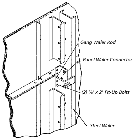
Panel Waler Connection
