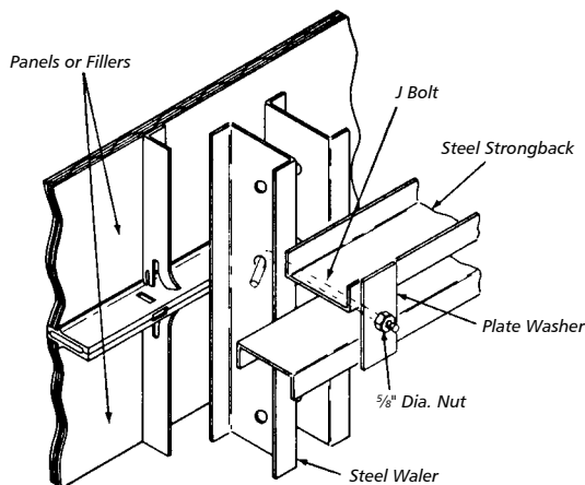
5" Versiform Walers Used as a Steel Strongback
