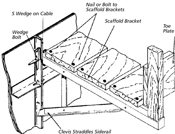
Scaffold Bracket Attachment
