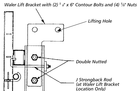
Double Duty Lift Bracket Attachment
